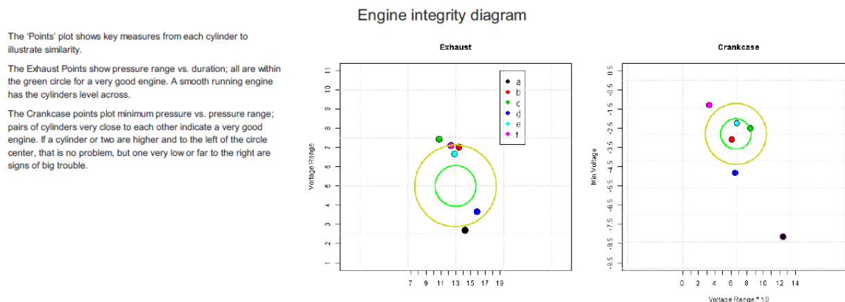
Figure 11: Engine Integrity diagram showing the (dis)similarity of the value of parameters for each cylinder derived from the Signature data.
