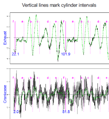
Figure 14: The Polygraph Model of the Pressure vs. vibration in the EP Signature for the subject engine.
